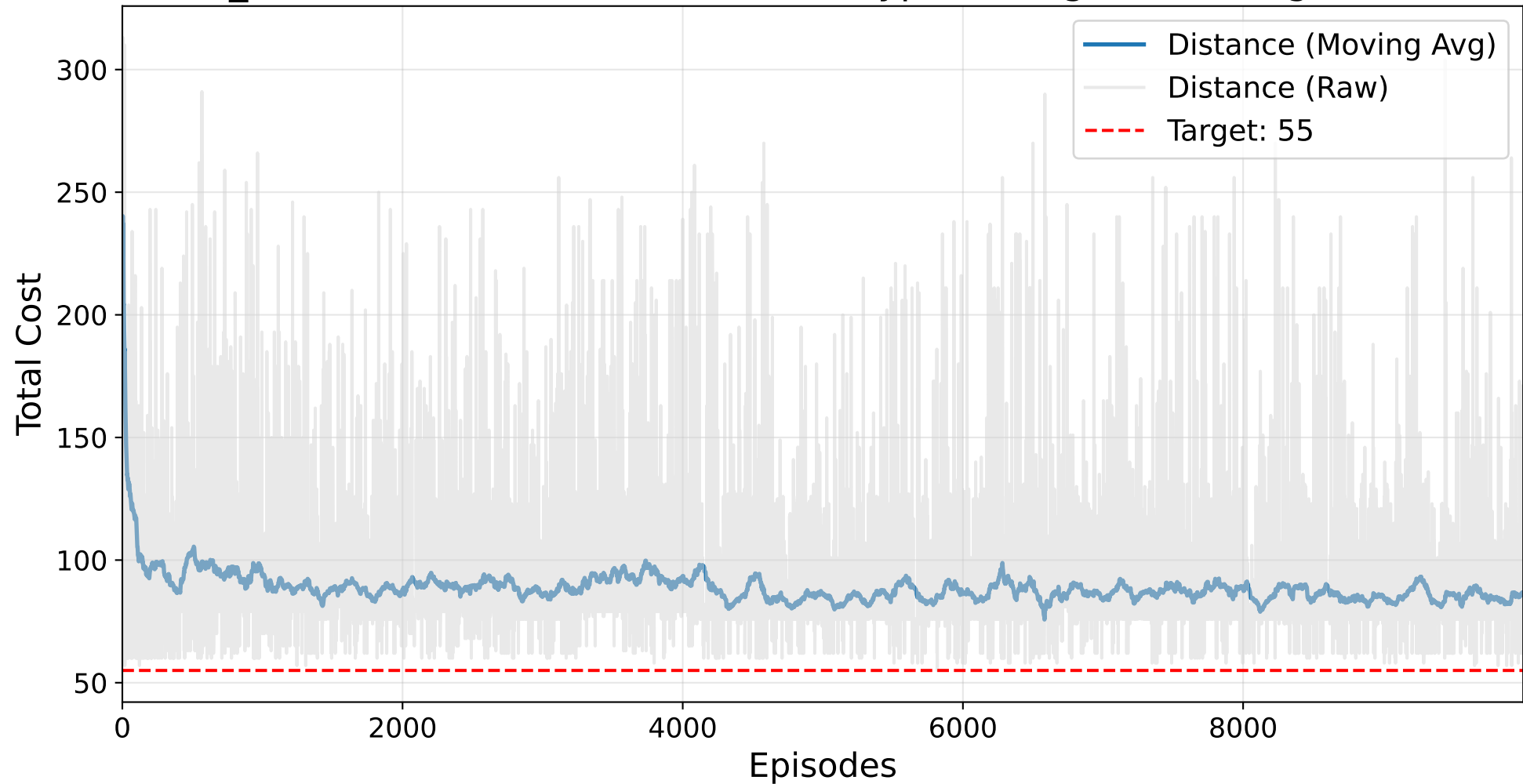
Final NO_BAYESIAN Masked AutoRL-SOP (HyperTuningSK) Training - br17.10.sop
